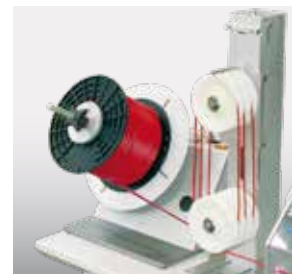
▲ ads 115 active de-reeler with wire reel
